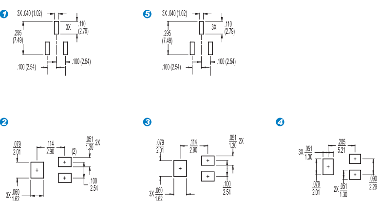
PC Board Patterns (PCB板孔尺寸图)
