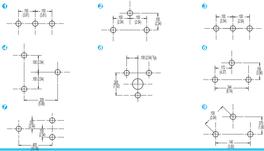
PC Board Patterns (PCB板孔尺寸图)
