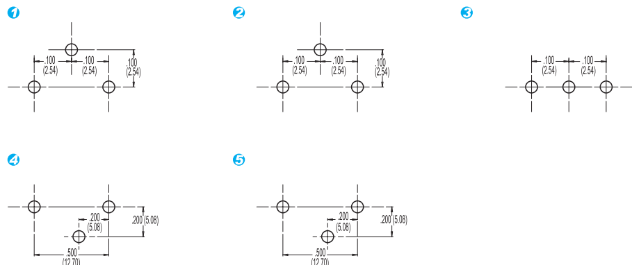
PC Board Patterns(PCB板孔尺寸图)
