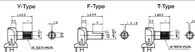
F-122K Series Shaft Dimensions and Styles
