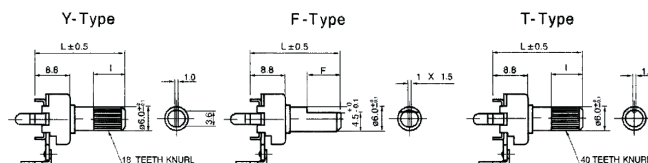
F-122K Series Shaft Dimensions and Styles
